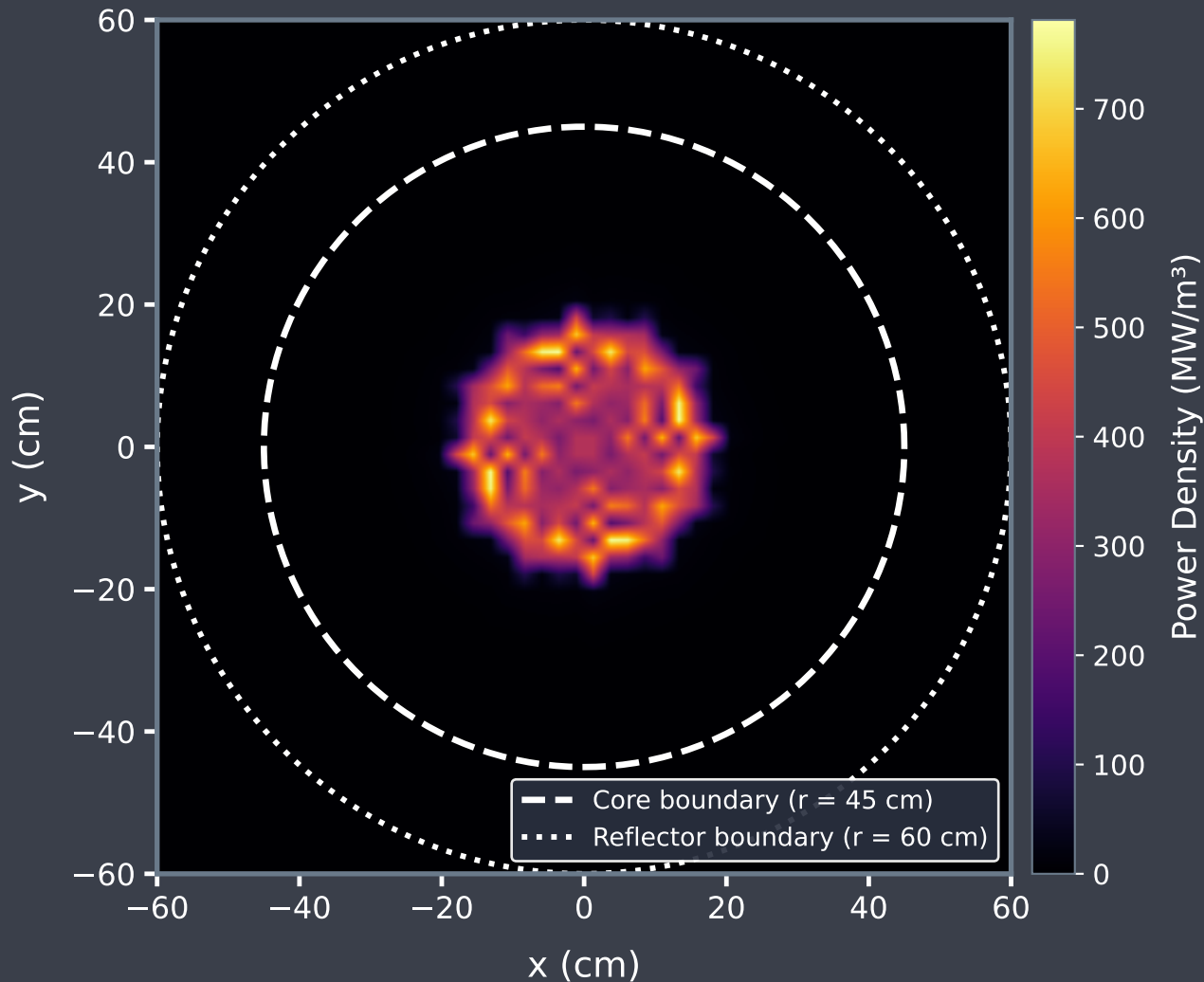
TRAVIS Core — Reconstructed Full-Core Radial Power (from 1/12 symmetry, at z = 0 )
